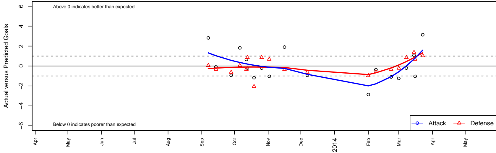
MRFC White B99 Dots are actual minus expected GF (blue circles) and GA (red triangles). Blue line is smoothed change in attack strength. Red is smoothed change in defense strength.
